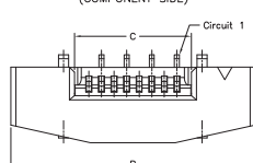
SUGGESTED PCB LAYOUT (COMPONENT SIDE)
